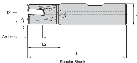
Regular Shank
