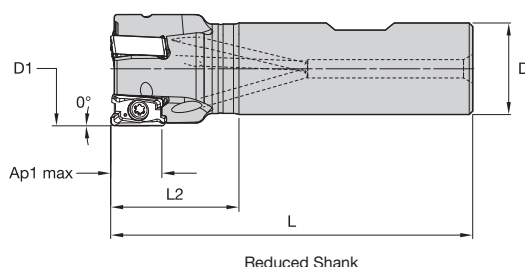
Reduced Shank
