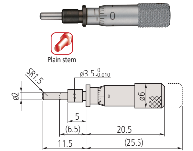
148-215 Mass: 4 g
